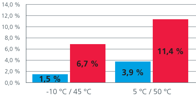
R404A HGX44e/475-4 vs. HGX4/465-4
