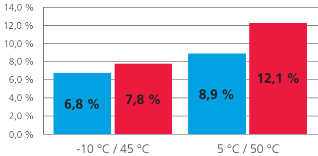
R404A HGX44e/770-4 S vs. HGX5/725-4 S
