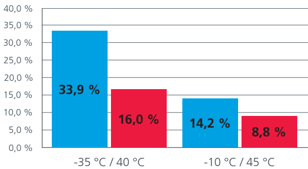
R404A HGX44e/770-4 S vs. HGX5/725-4 S
