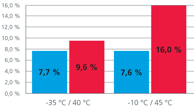
R404A HGX44e/475-4 vs. HGX4/465-4
